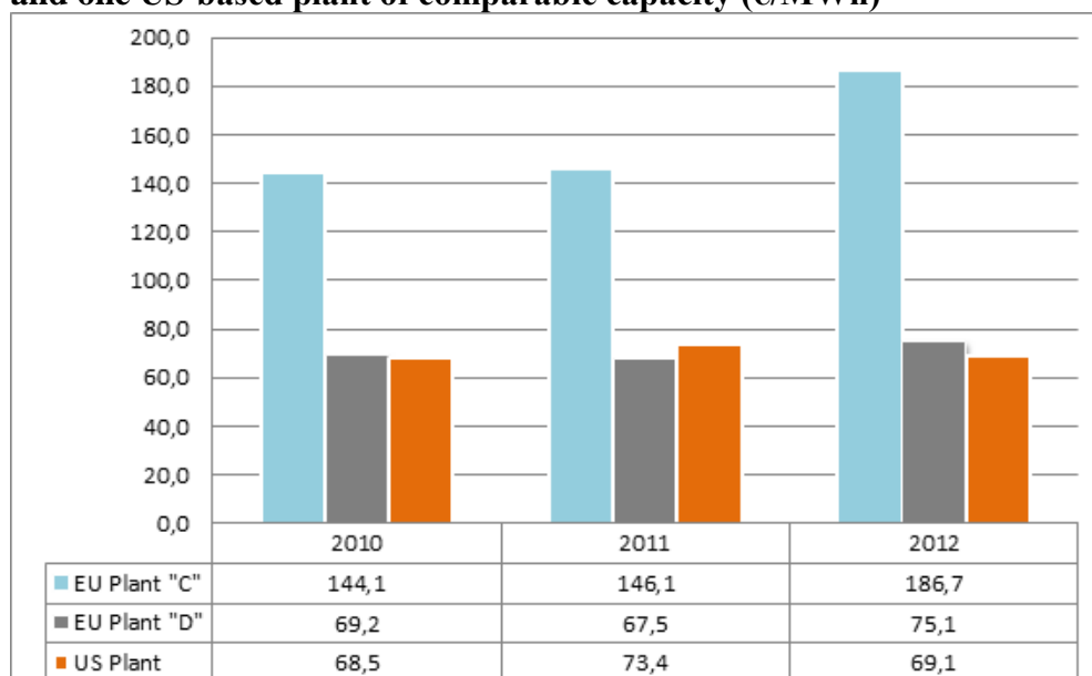
Figure 138 Prices of electricity: comparison of two EU-based brick and roof tile plants and one US-based plant of comparable capacity (€/MWh)
